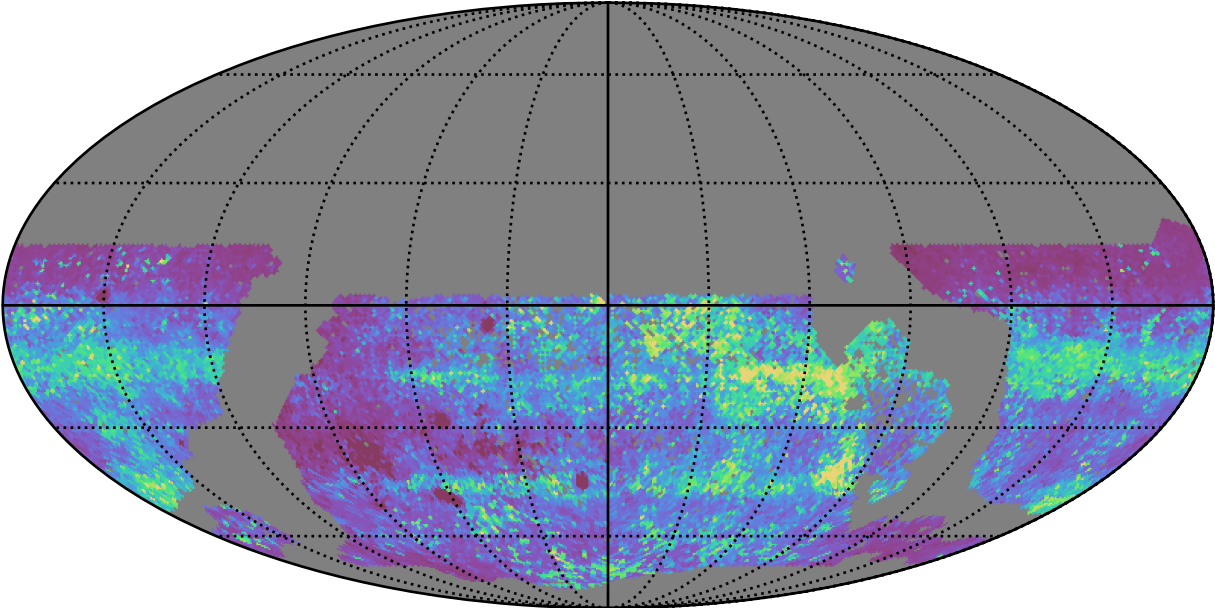
too_elab_heavy_r128_d2_griz_v3.4_10yrs WFD zy bands: 75th Percentile Intranight Timespan
