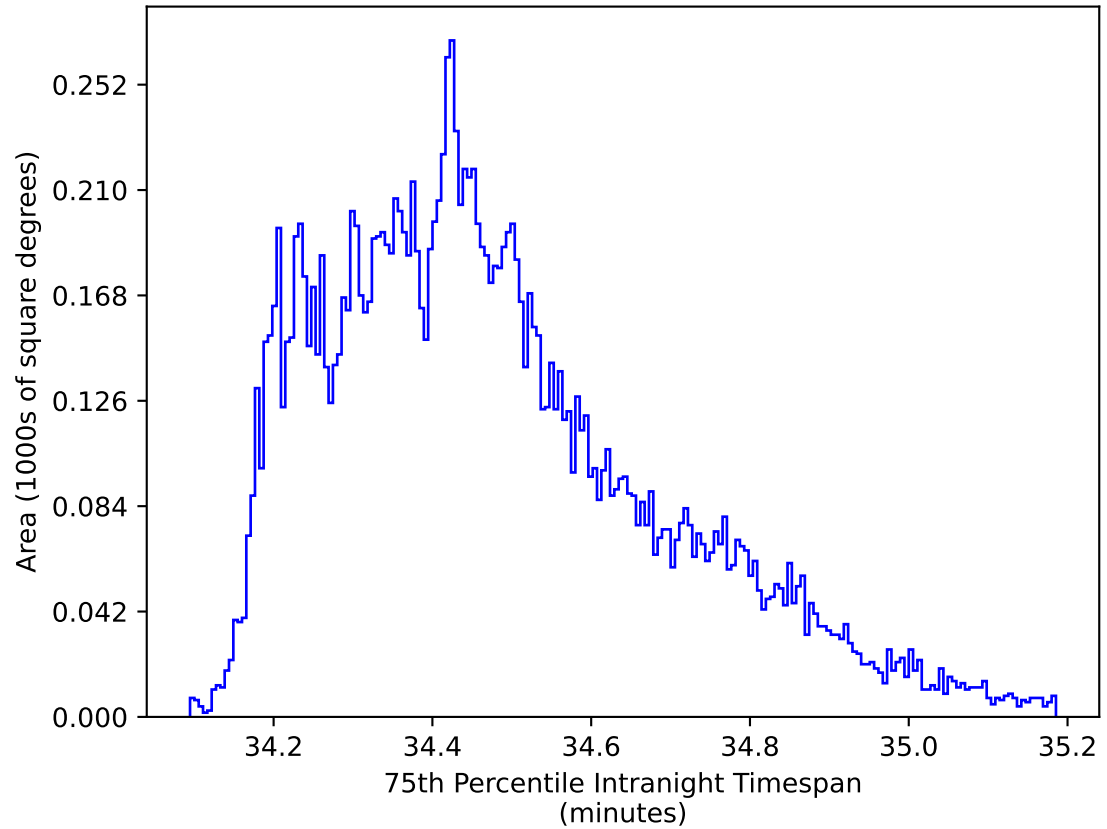
too_elab_heavy_r128_d2_griz_v3.4_10yrs WFD zy bands: 75th Percentile Intranight Timespan
