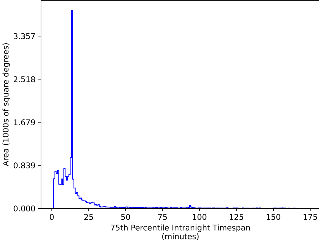
too_elab_heavy_r128_d2_griz_v3.4_10yrs WFD z band: 75th Percentile Intranight Timespan
