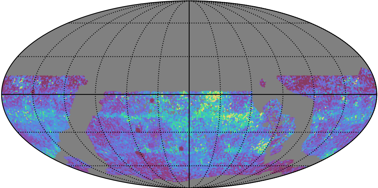
too_elab_heavy_r128_d2_griz_v3.4_10yrs WFD y band: 75th Percentile Intranight Timespan
