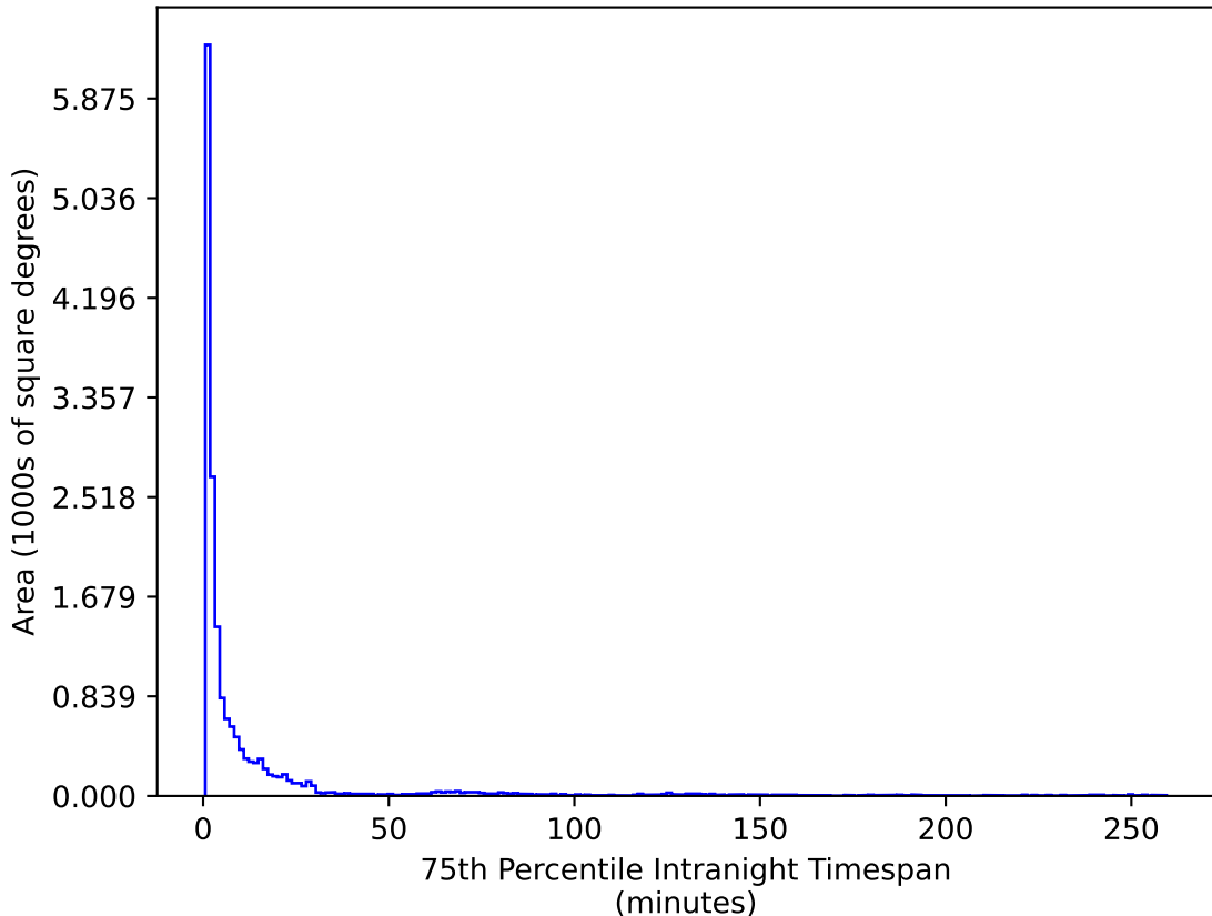
too_elab_heavy_r128_d2_griz_v3.4_10yrs WFD u band: 75th Percentile Intranight Timespan
