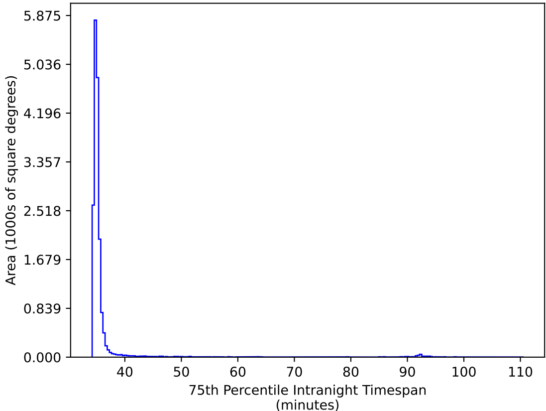
too_elab_heavy_r128_d2_griz_v3.4_10yrs WFD ri bands: 75th Percentile Intranight Timespan
