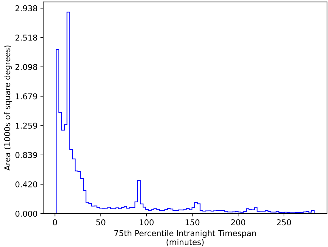
too_elab_heavy_r128_d2_griz_v3.4_10yrs WFD r band: 75th Percentile Intranight Timespan
