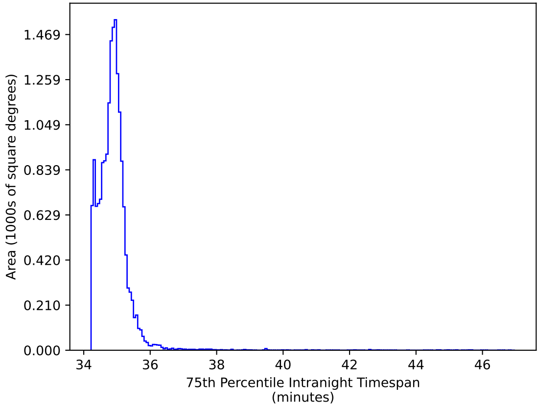
too_elab_heavy_r128_d2_griz_v3.4_10yrs WFD iz bands: 75th Percentile Intranight Timespan
