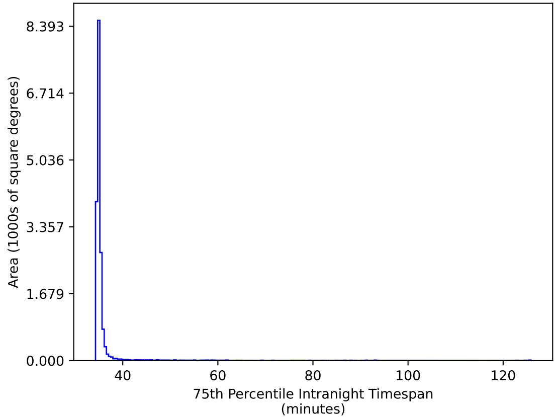
too_elab_heavy_r128_d2_griz_v3.4_10yrs WFD gr bands: 75th Percentile Intranight Timespan
