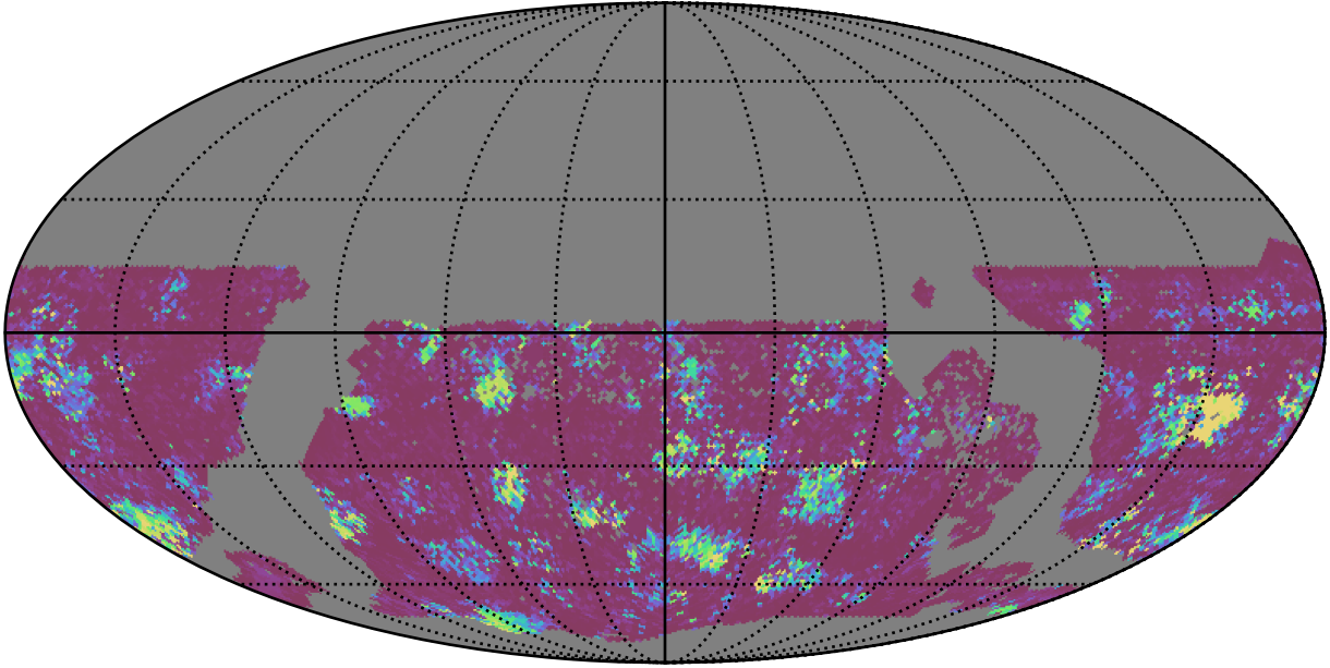
too_elab_heavy_r128_d2_griz_v3.4_10yrs WFD g band: 75th Percentile Intranight Timespan
