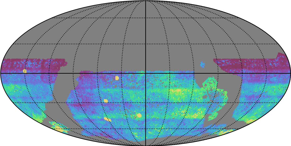
too_elab_heavy_r128_d2_griz_v3.4_10yrs WFD all bands: 75th Percentile Intranight Timespan
