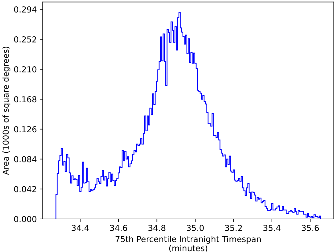
too_elab_heavy_r128_d2_griz_v3.4_10yrs WFD all bands: 75th Percentile Intranight Timespan
