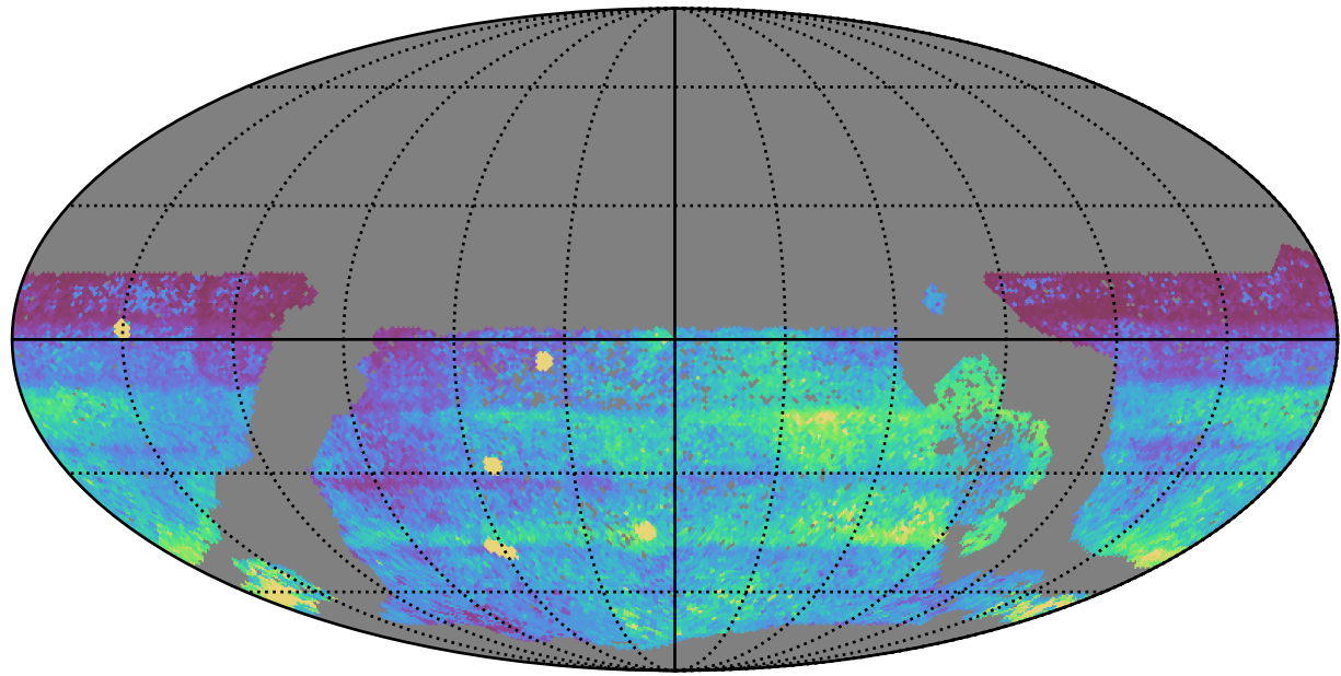
too_elab_heavy_r128_d2_griz_v3.4_10yrs WFD: 75th Percentile Intranight Timespan
