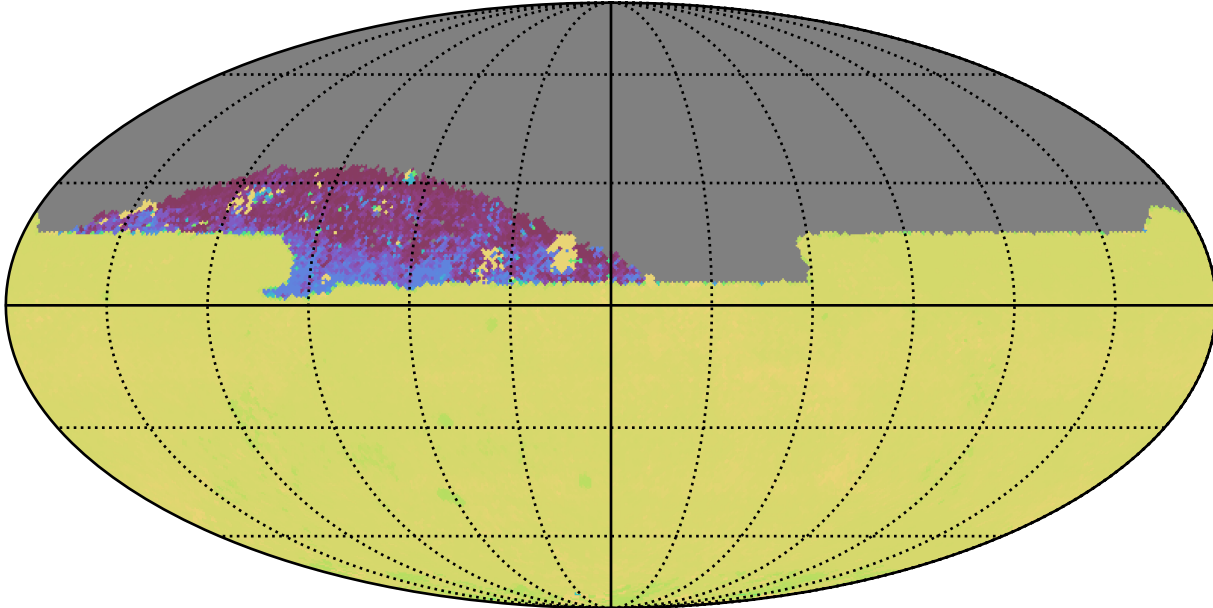
too_elab_heavy_r128_d2_griz_v3.4_10yrs All sky zy bands: 75th Percentile Intranight Timespan
