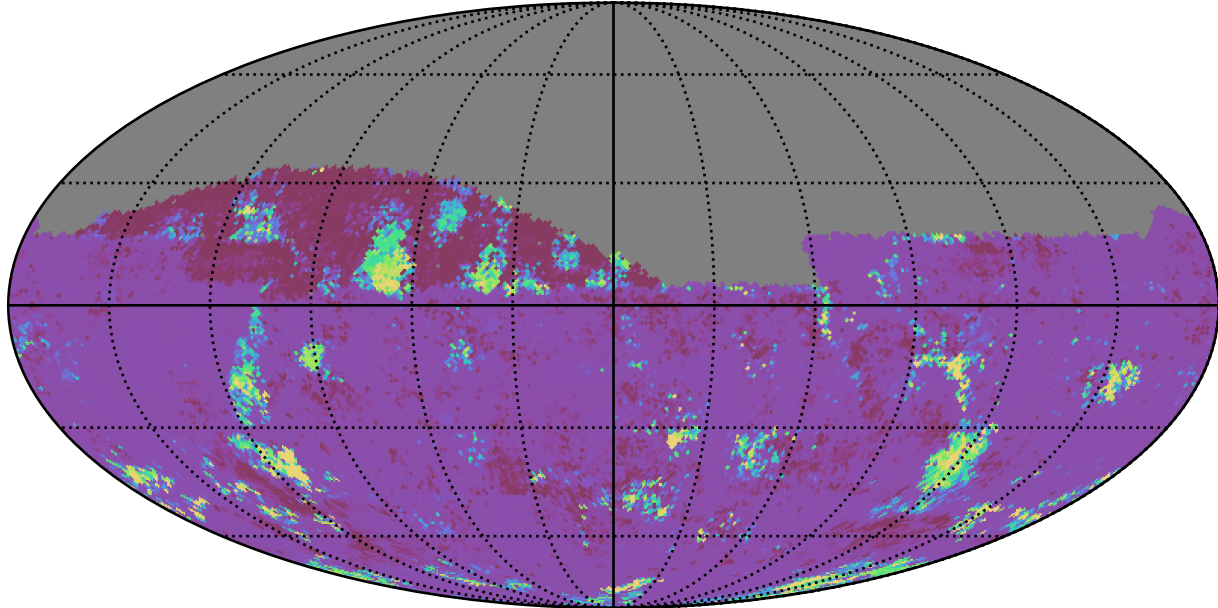
too_elab_heavy_r128_d2_griz_v3.4_10yrs All sky ug bands: 75th Percentile Intranight Timespan
