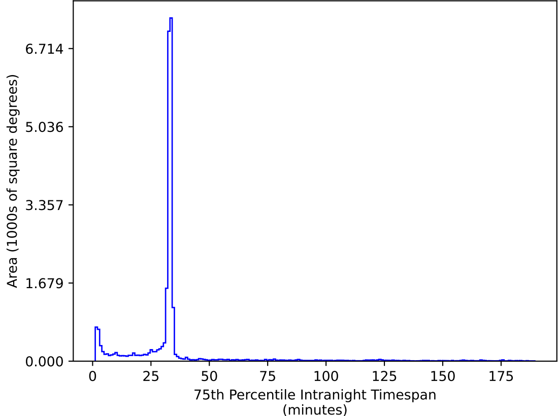
too_elab_heavy_r128_d2_griz_v3.4_10yrs All sky ug bands: 75th Percentile Intranight Timespan
