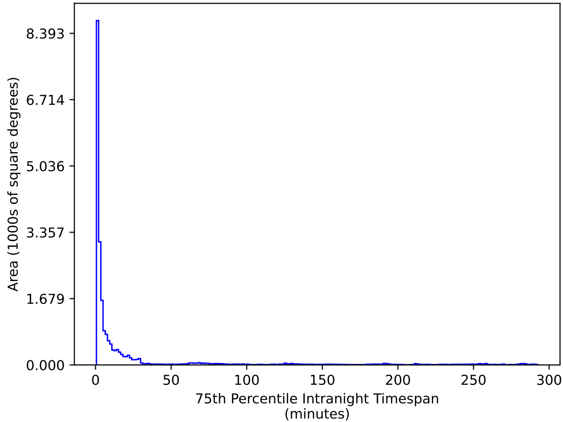
too_elab_heavy_r128_d2_griz_v3.4_10yrs All sky u band: 75th Percentile Intranight Timespan
