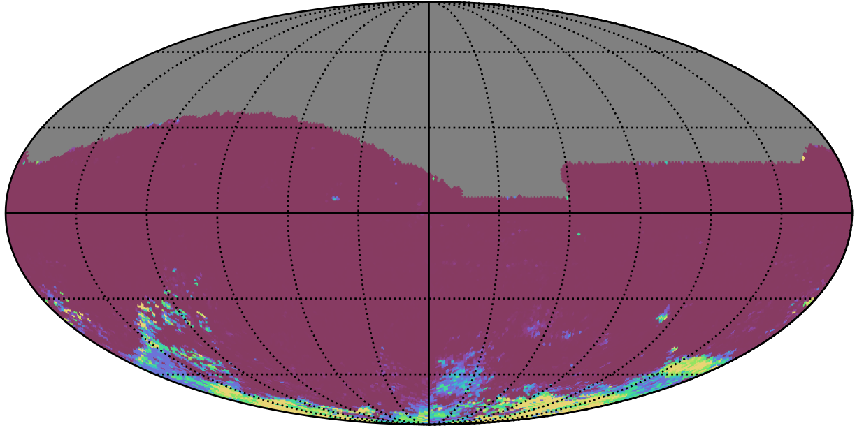
too_elab_heavy_r128_d2_griz_v3.4_10yrs All sky ri bands: 75th Percentile Intranight Timespan
