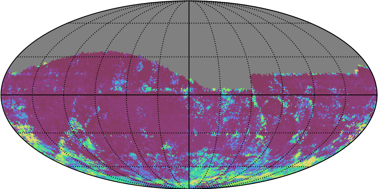
too_elab_heavy_r128_d2_griz_v3.4_10yrs All sky i band: 75th Percentile Intranight Timespan
