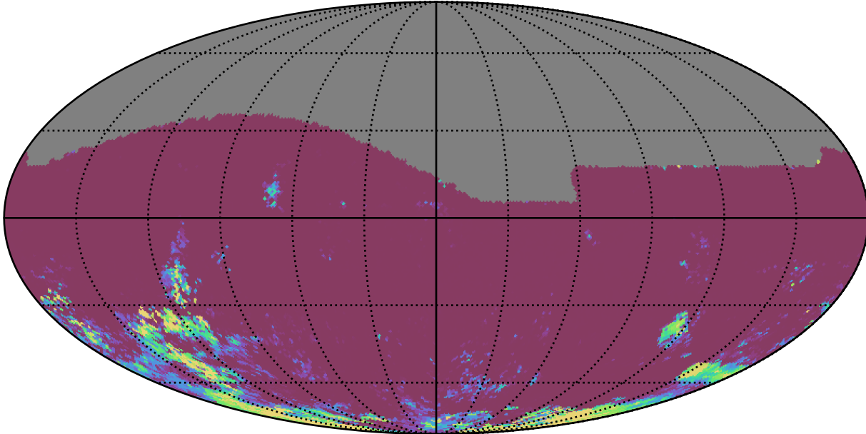
too_elab_heavy_r128_d2_griz_v3.4_10yrs All sky gr bands: 75th Percentile Intranight Timespan
