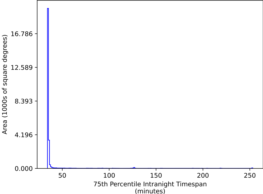
too_elab_heavy_r128_d2_griz_v3.4_10yrs All sky gr bands: 75th Percentile Intranight Timespan
