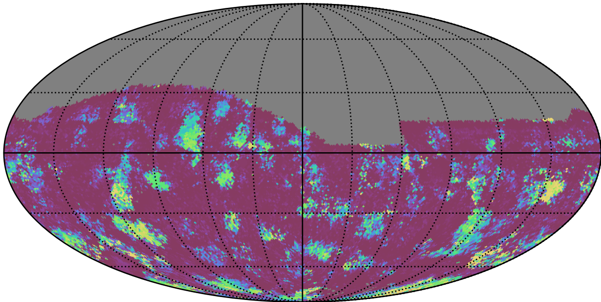
too_elab_heavy_r128_d2_griz_v3.4_10yrs All sky g band: 75th Percentile Intranight Timespan
