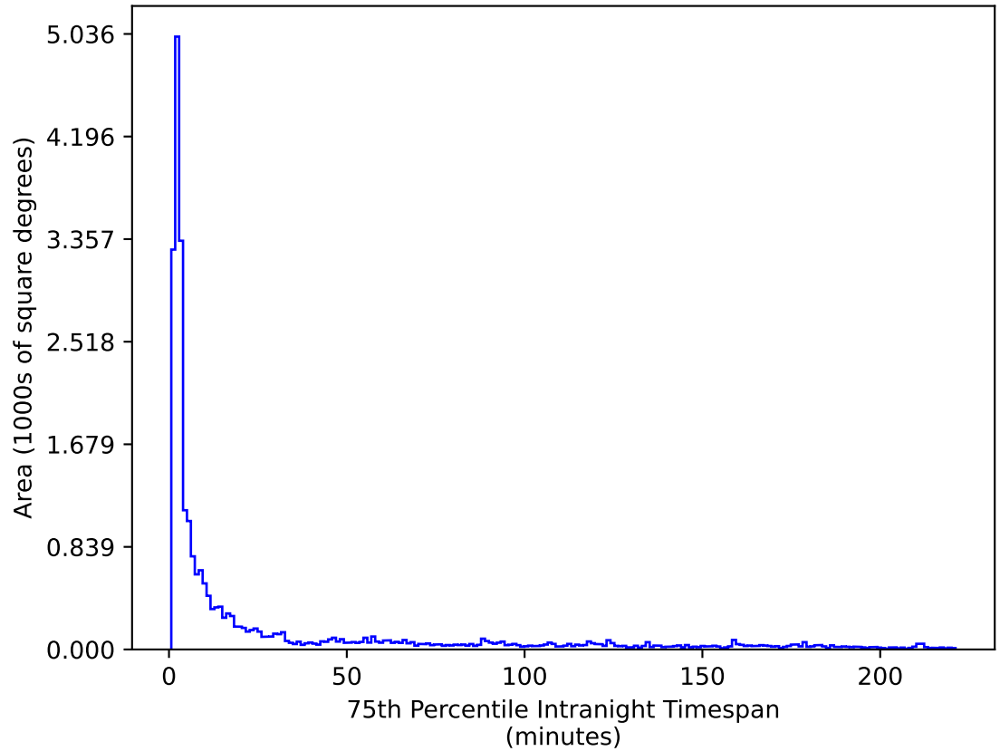
too_elab_heavy_r128_d2_griz_v3.4_10yrs All sky g band: 75th Percentile Intranight Timespan
