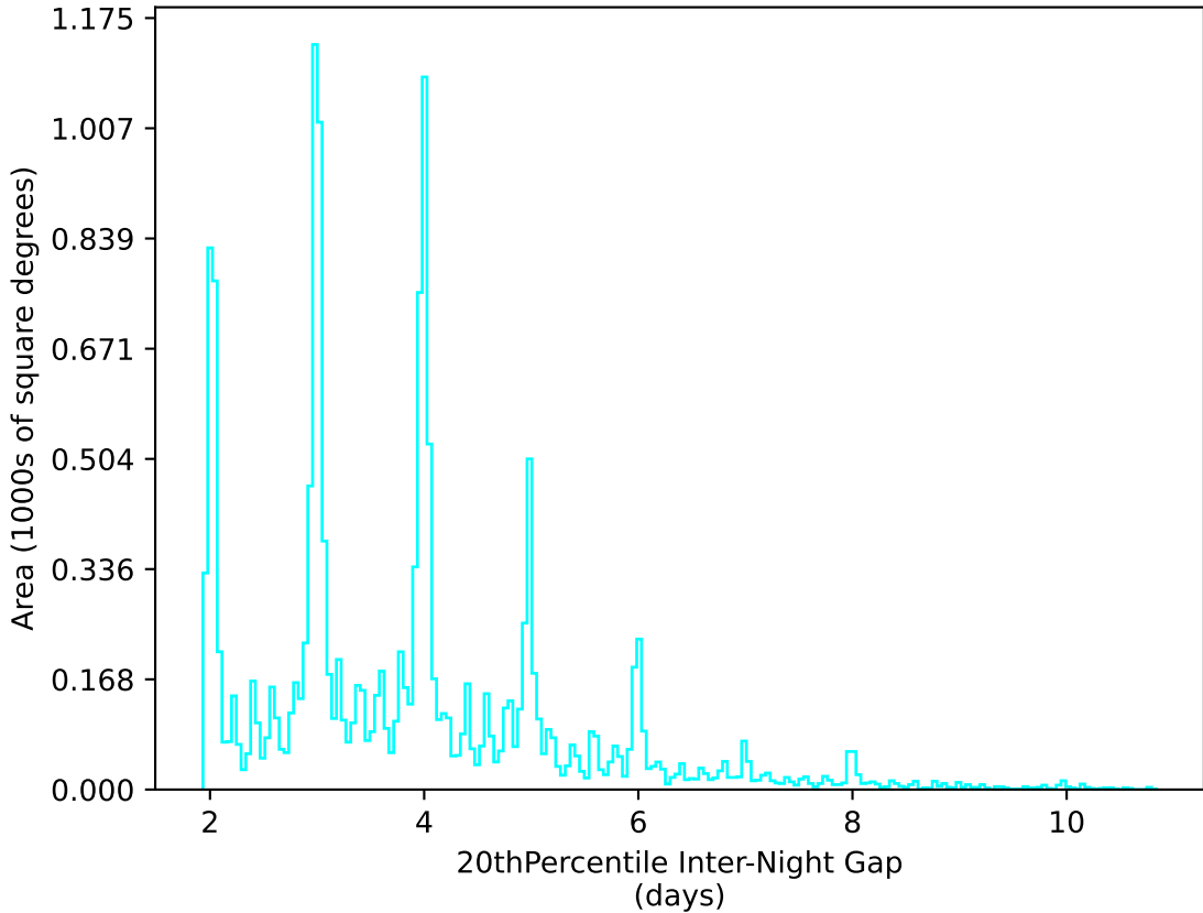
too_elab_heavy_r128_d2_griz_v3.4_10yrs WFD u band: 20thPercentile Inter-Night Gap
