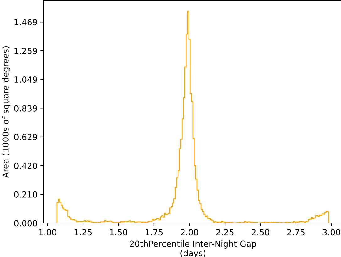
too_elab_heavy_r128_d2_griz_v3.4_10yrs WFD r band: 20thPercentile Inter-Night Gap
