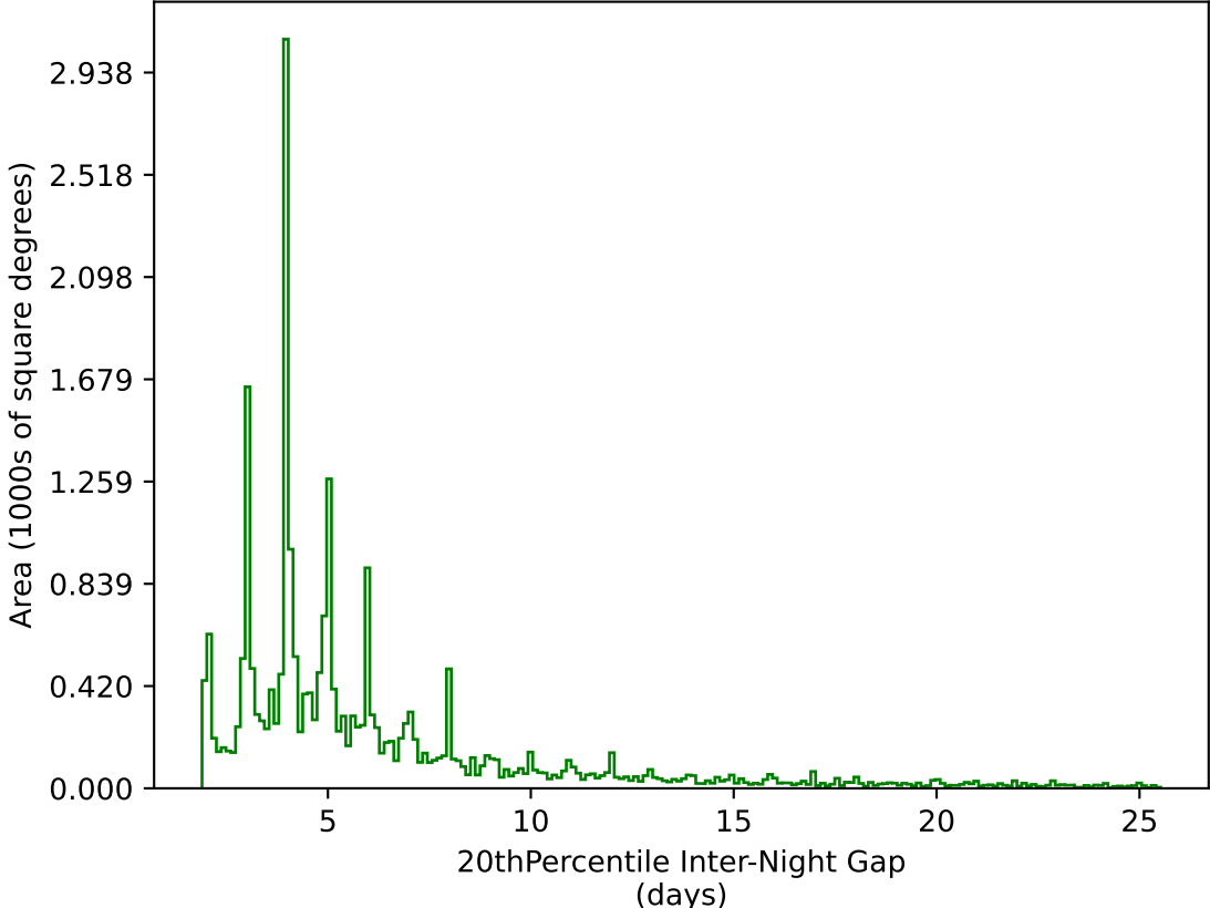
too_elab_heavy_r128_d2_griz_v3.4_10yrs All sky g band: 20thPercentile Inter-Night Gap
