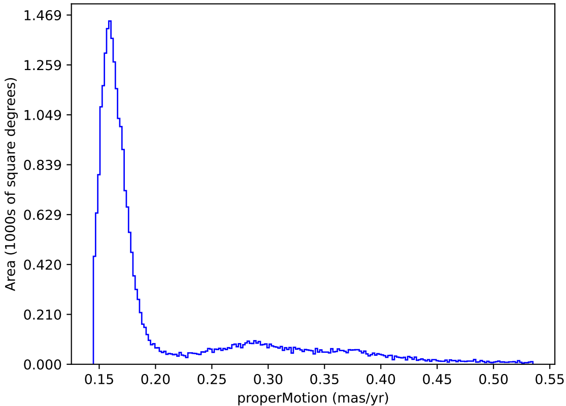
too_elab_heavy_r128_d2_griz_v3.4_10yrs : properMotion
