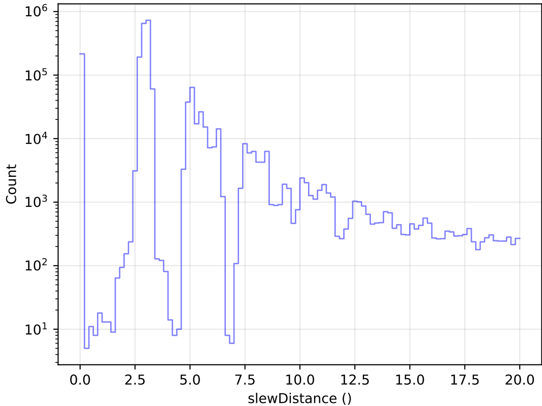
too_elab_heavy_r128_d2_griz_v3.4_10yrs All visits: Zoom Slew Distance Histogram
