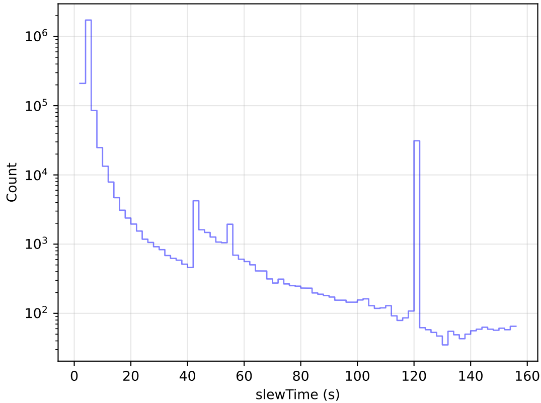
too_elab_heavy_r128_d2_griz_v3.4_10yrs All visits: Slew Time Histogram
