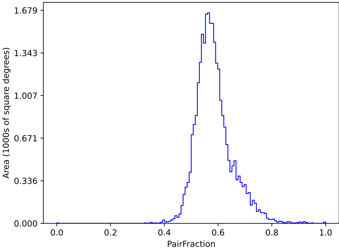
too_elab_heavy_r128_d2_griz_v3.4_10yrs (g or r or i): PairFraction
