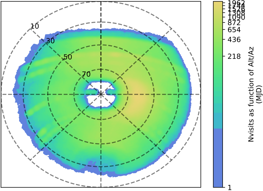
too_elab_heavy_r128_d2_griz_v3.4_10yrs y: Nvisits as function of Alt/Az
