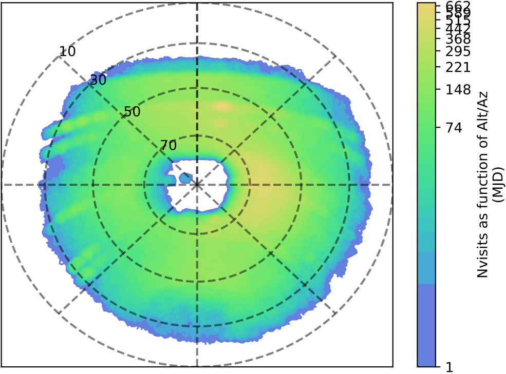
too_elab_heavy_r128_d2_griz_v3.4_10yrs u: Nvisits as function of Alt/Az
