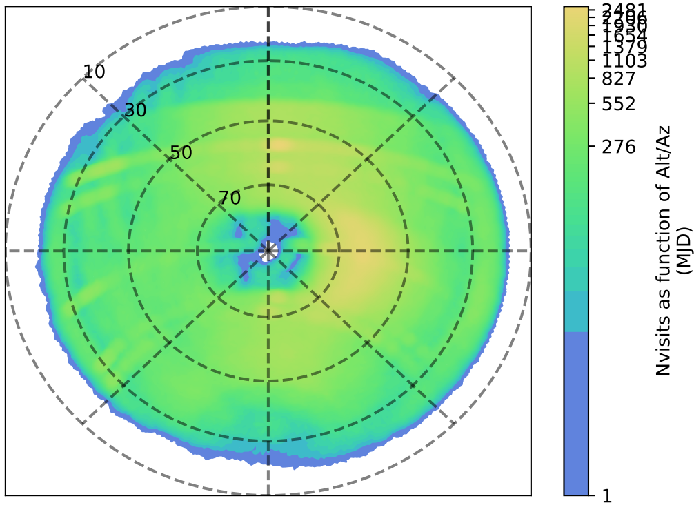
too_elab_heavy_r128_d2_griz_v3.4_10yrs i: Nvisits as function of Alt/Az
