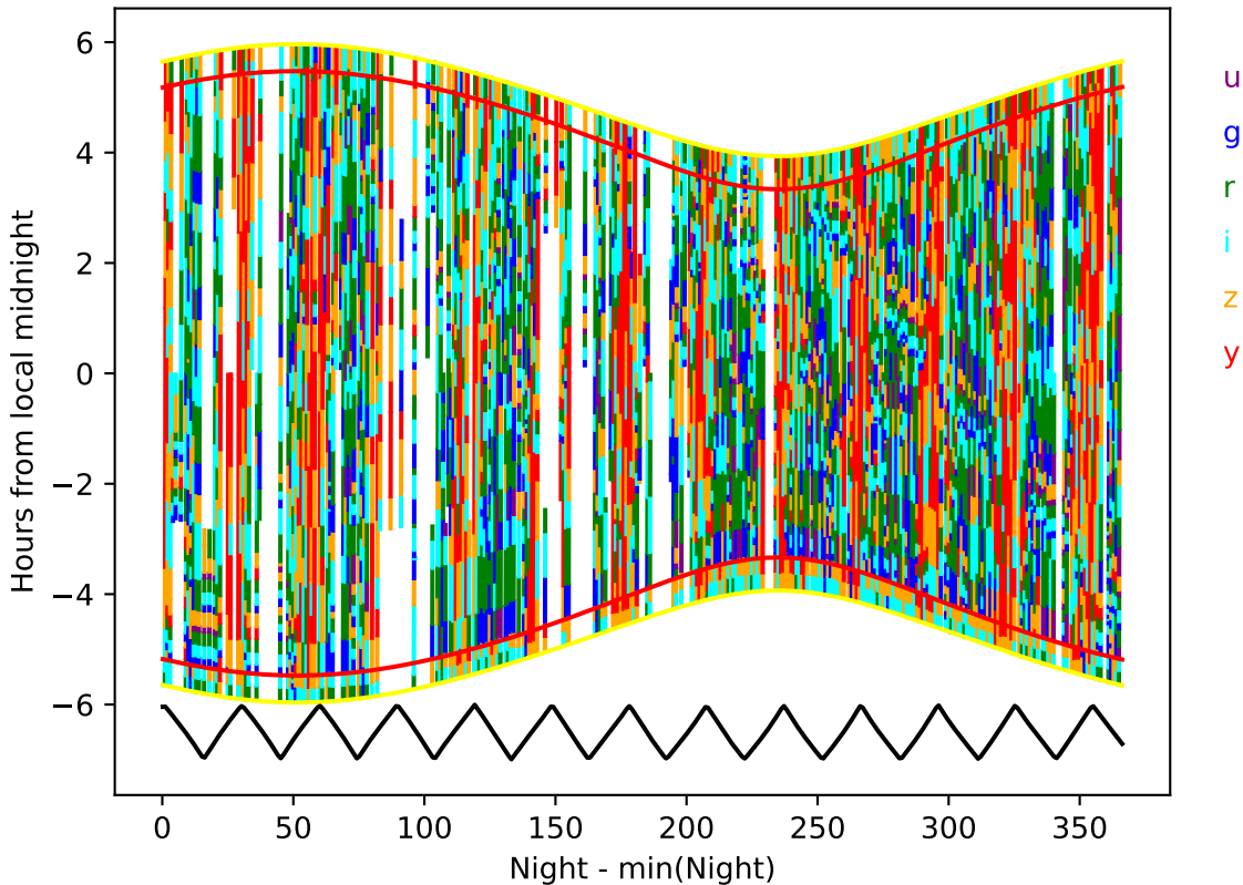
too_elab_heavy_r128_d2_griz_v3.4_10yrs year 1-2: Hourglass
