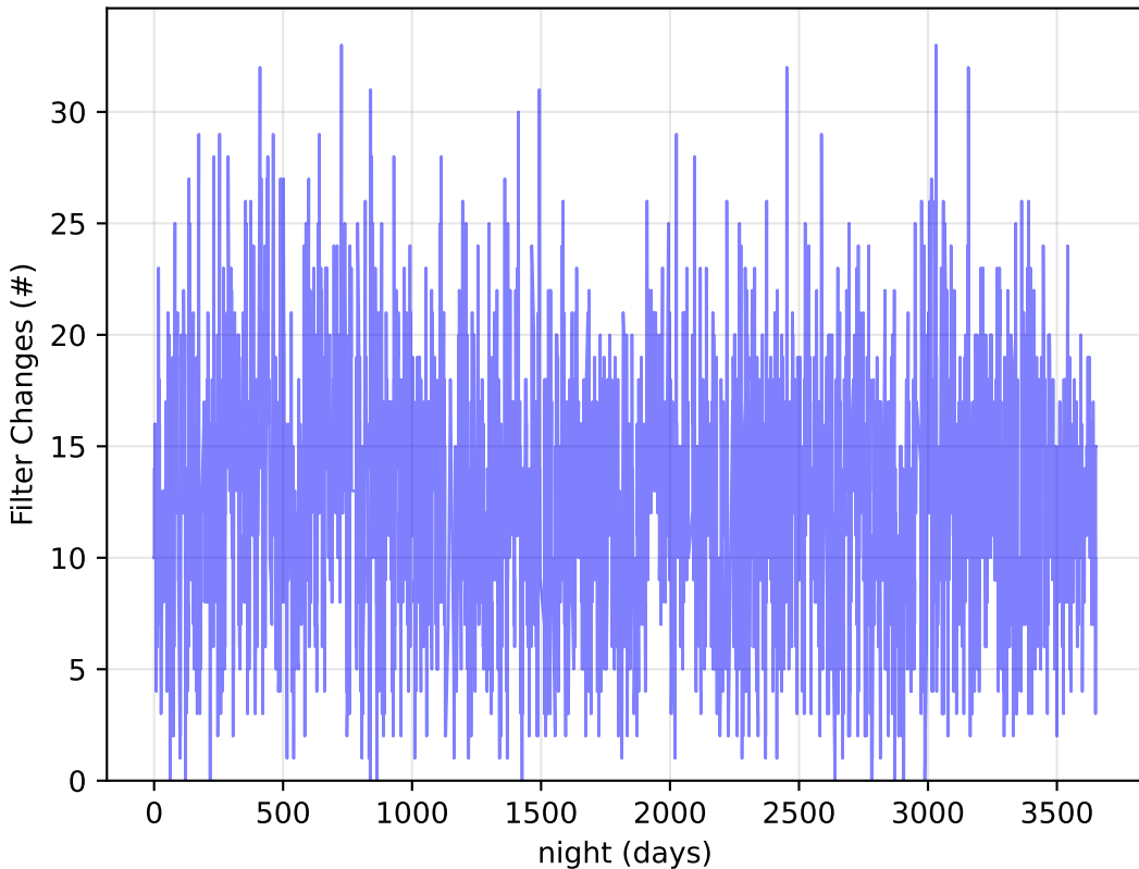
too_elab_heavy_r128_d2_griz_v3.4_10yrs : Filter Changes
