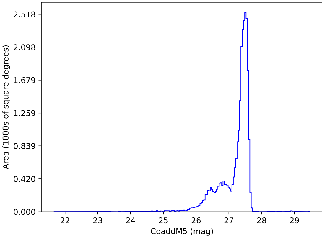
too_elab_heavy_r128_d2_griz_v3.4_10yrs : CoaddM5
