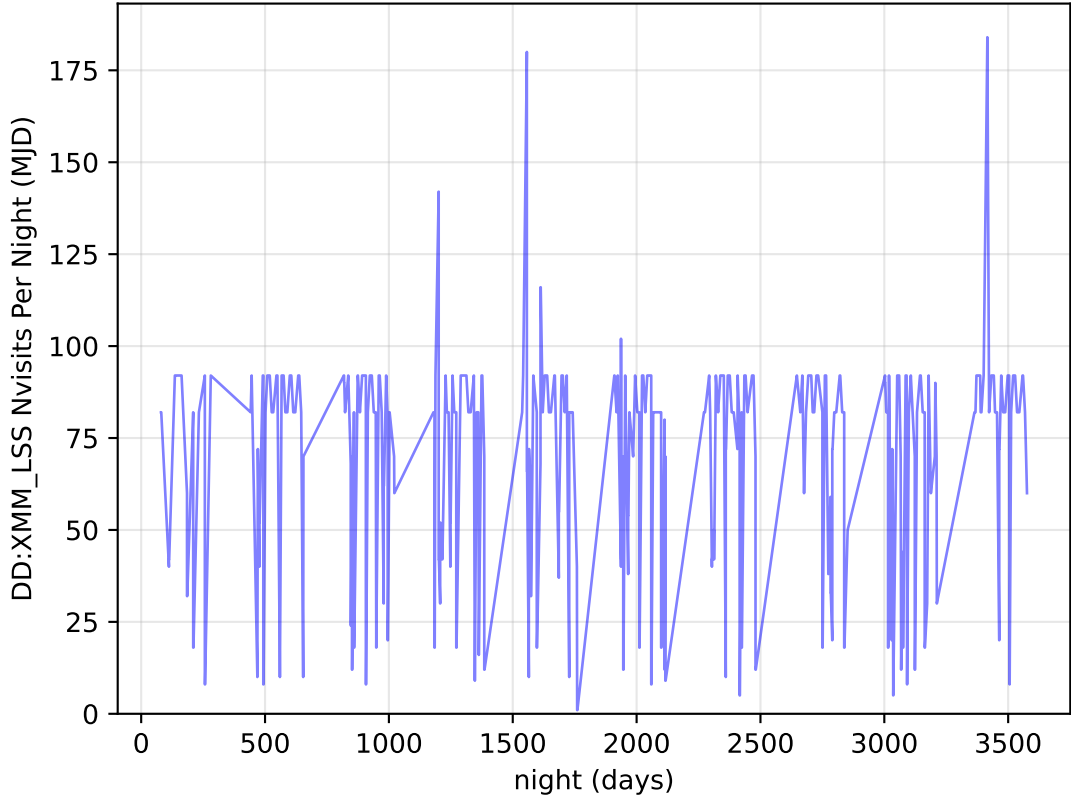
too_elab_heavy_r128_d2_griz_v3.4_10yrs all bands: DD:XMM_LSS Nvisits Per Night
