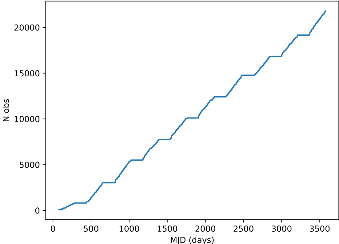
too_elab_heavy_r128_d2_griz_v3.4_10yrs all bands: DD:XMM_LSS Cumulative NVisits
