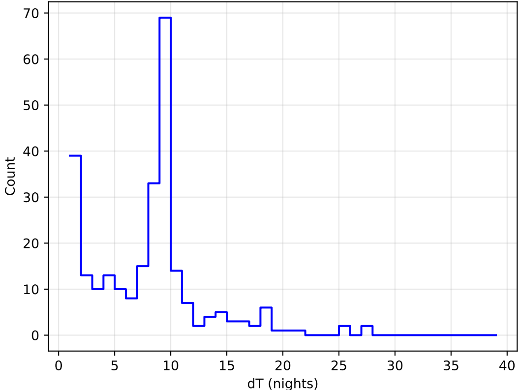
too_elab_heavy_r128_d2_griz_v3.4_10yrs all bands: DD:ELAISS1 Delta Nights Histogram
