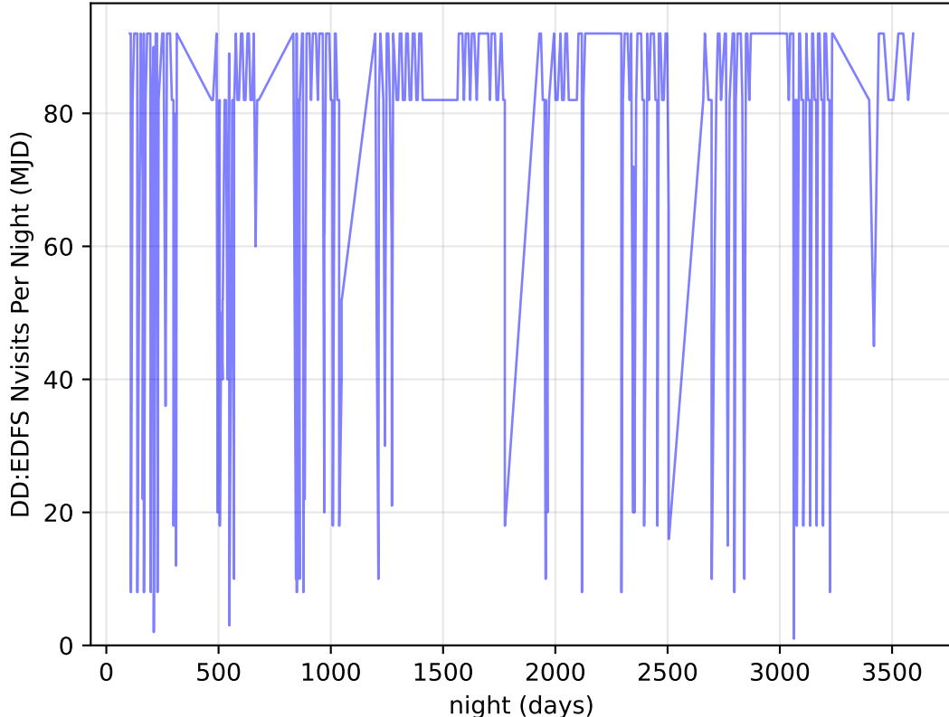
too_elab_heavy_r128_d2_griz_v3.4_10yrs all bands: DD:EDFS Nvisits Per Night
