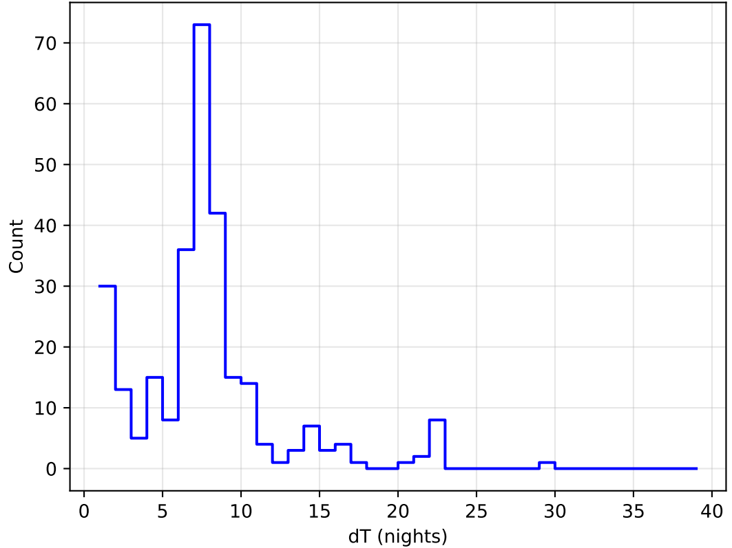
too_elab_heavy_r128_d2_griz_v3.4_10yrs all bands: DD:EDFS Delta Nights Histogram
