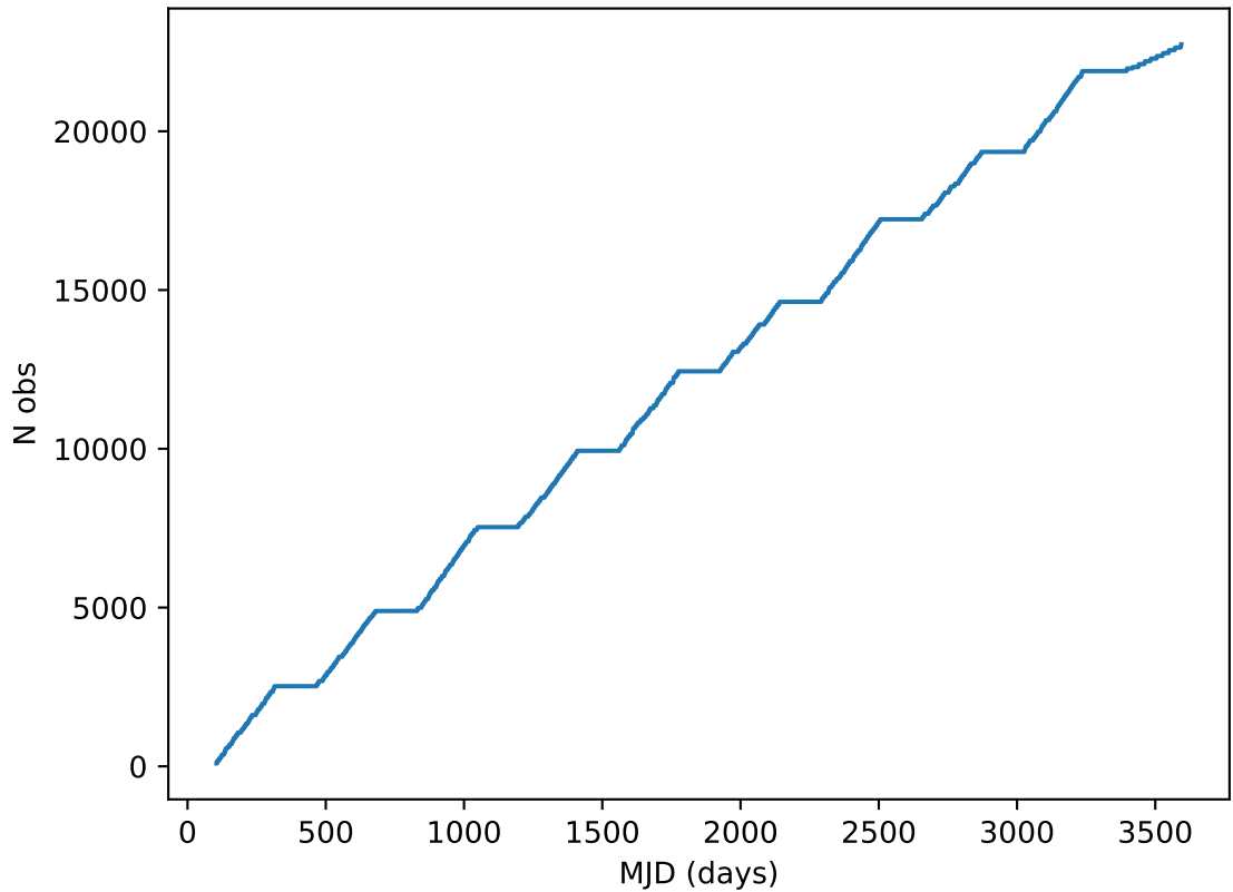
too_elab_heavy_r128_d2_griz_v3.4_10yrs all bands: DD:EDFS Cumulative NVisits
