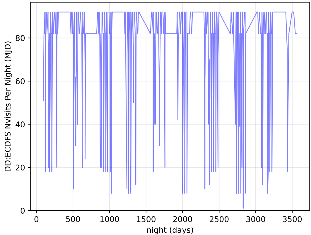
too_elab_heavy_r128_d2_griz_v3.4_10yrs all bands: DD:ECDFS Nvisits Per Night
