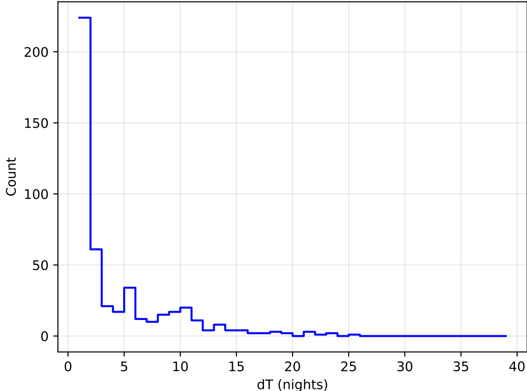
too_elab_heavy_r128_d2_griz_v3.4_10yrs all bands: DD: COSMOS Delta Nights Histogram
