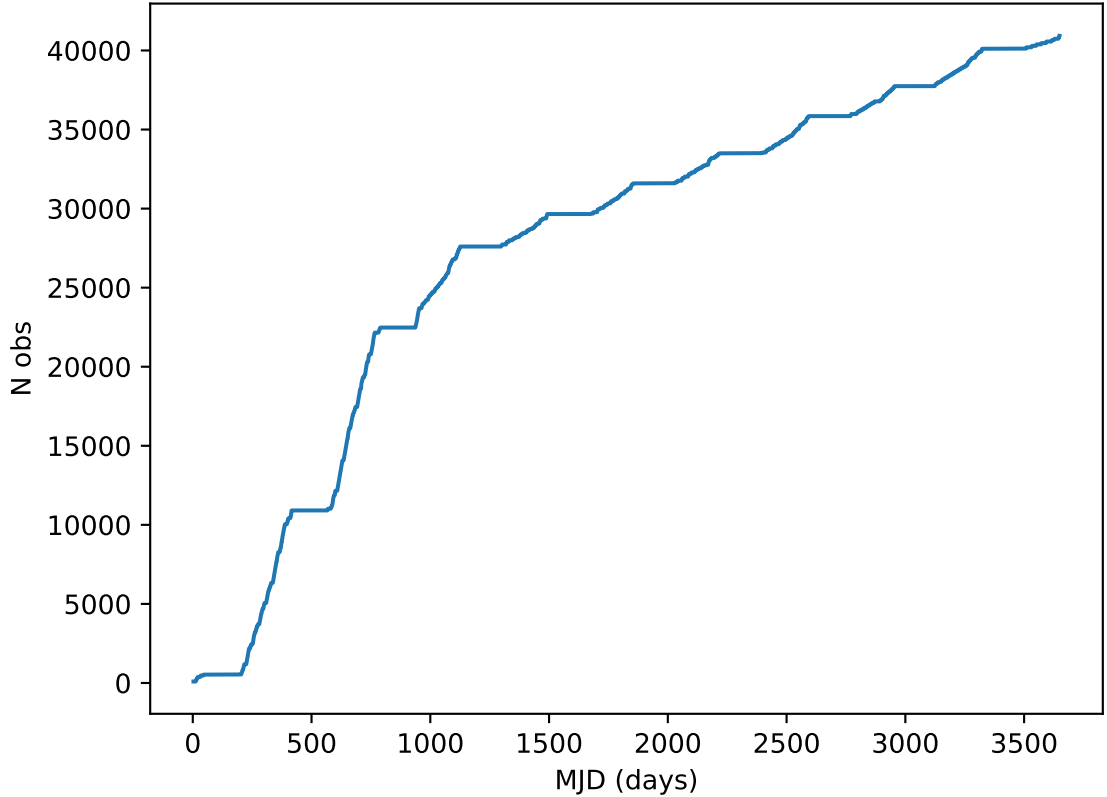
too_elab_heavy_r128_d2_griz_v3.4_10yrs all bands: DD: COSMOS Cumulative NVisits
