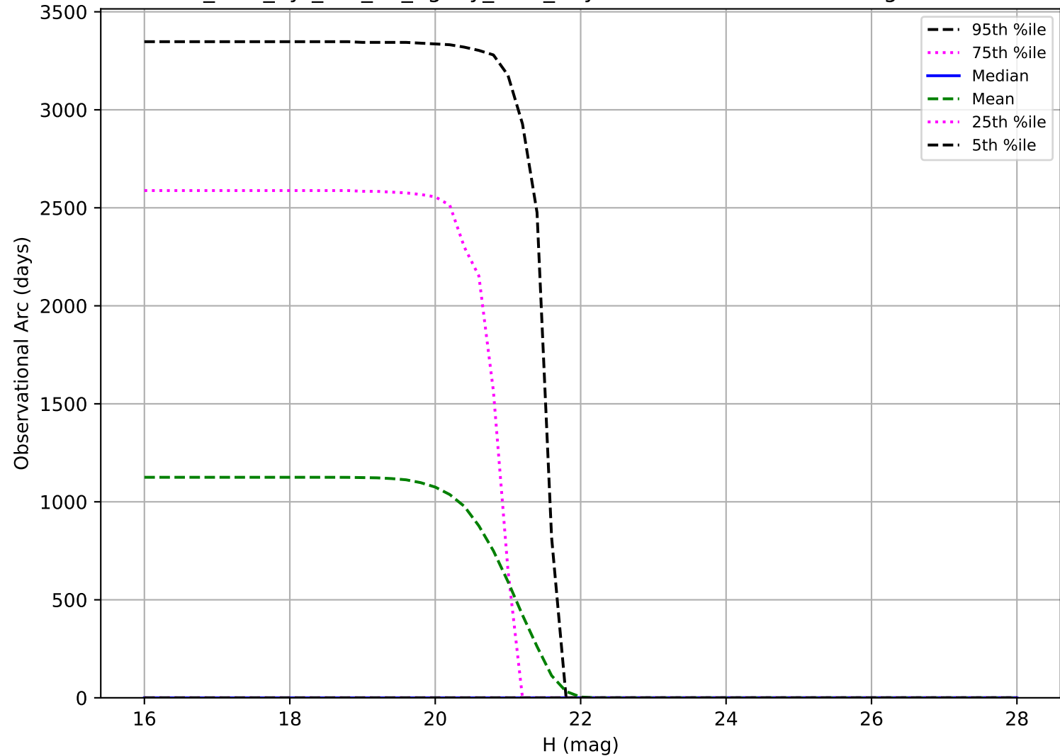
too_elab_2yr_r64_d3_ugrizy_v3.4_10yrs: Observational Arc Length Vatira
