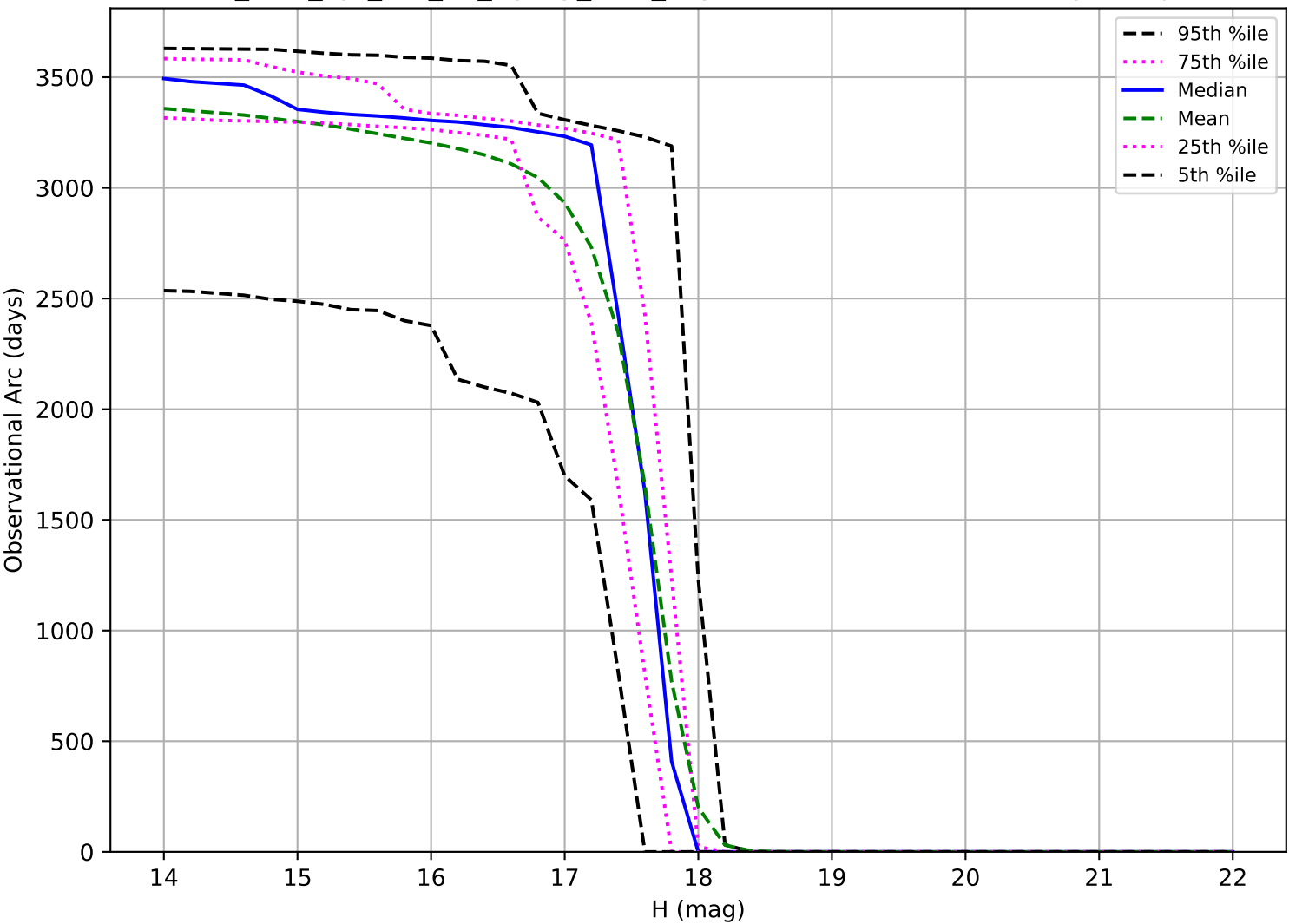
too_elab_2yr_r64_d3_ugrizy_v3.4_10yrs: Observational Arc Length Trojan
