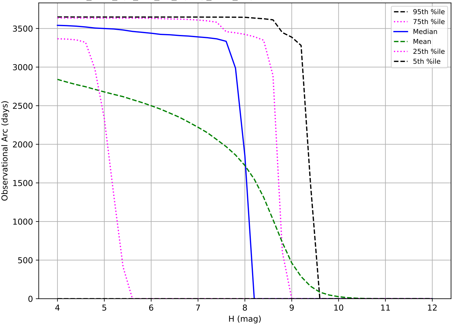
too_elab_2yr_r64_d3_ugrizy_v3.4_10yrs: Observational Arc Length TNO
