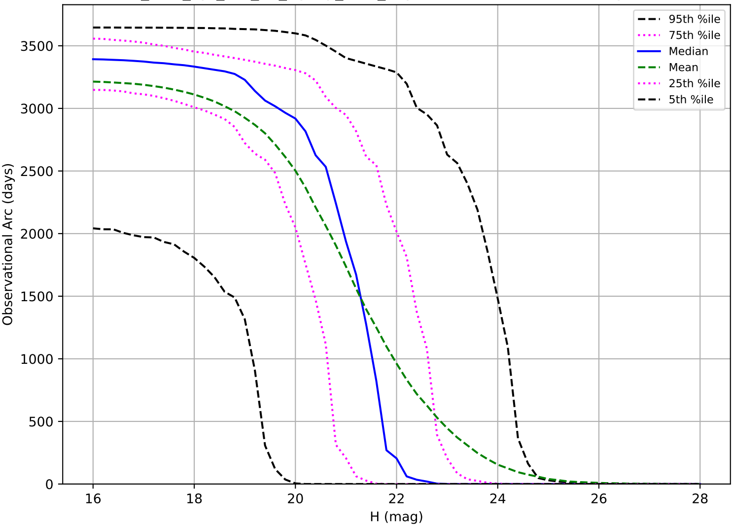
too_elab_2yr_r64_d3_ugrizy_v3.4_10yrs: Observational Arc Length PHA
