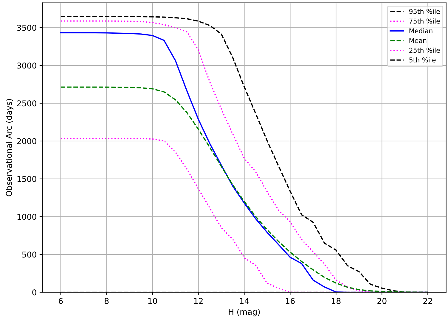
too_elab_2yr_r64_d3_ugrizy_v3.4_10yrs: Observational Arc Length OCC_r5
